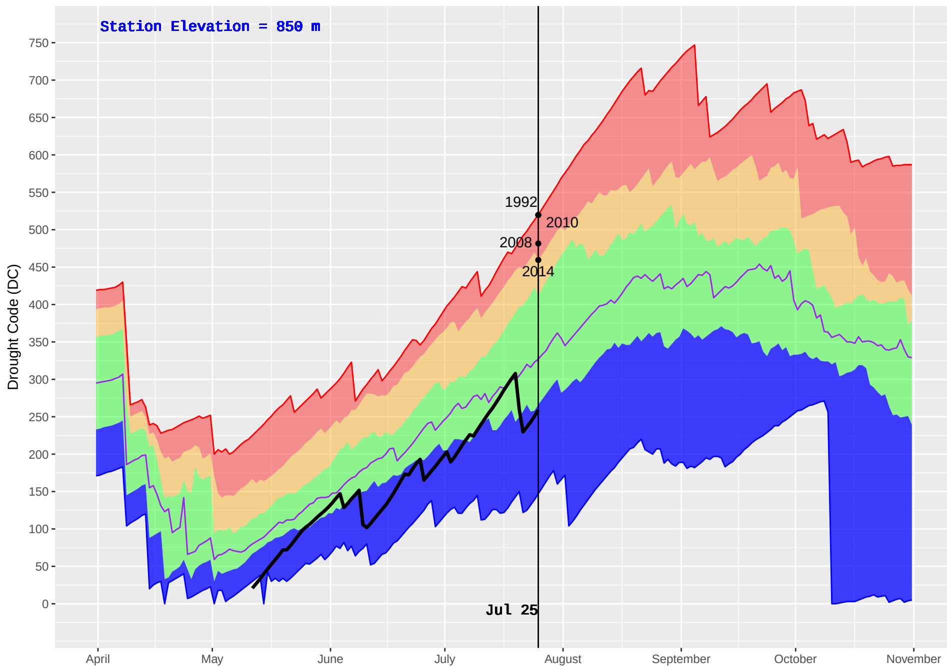
NORTH CHILCO (159) : Historical (1972–2016) and Current (2018) Noon Drought Code (DC)
